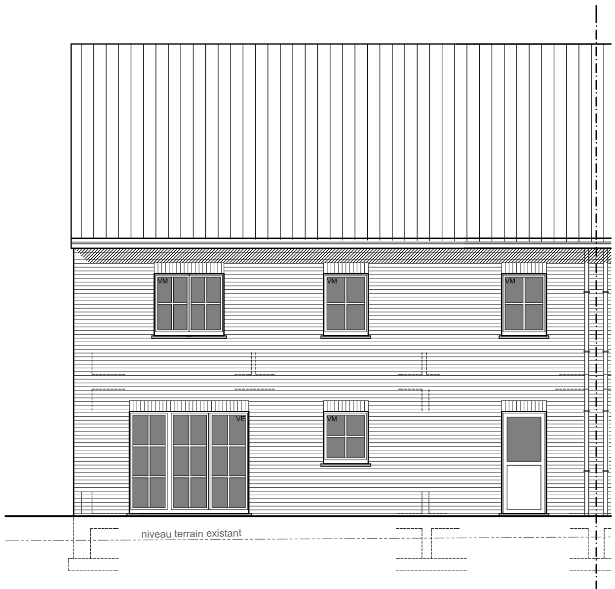
FACADE ARRIERE
